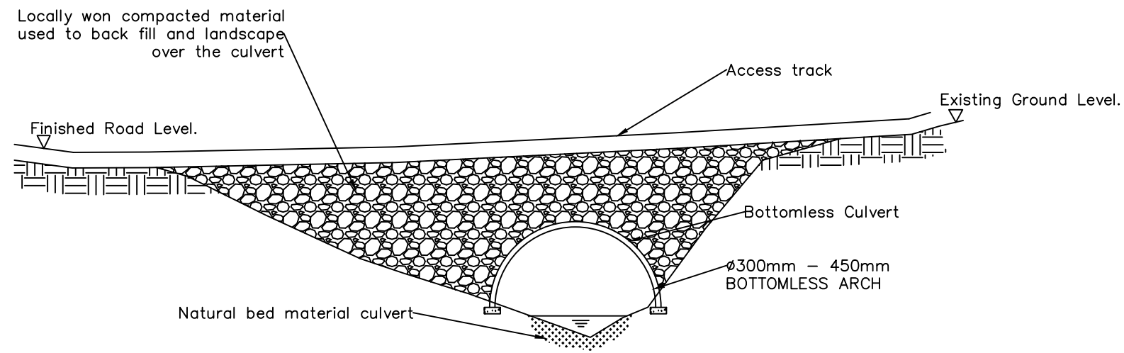
INDICATIVE BOTTOMLESS ARCH WATERCOURSE CROSSING
